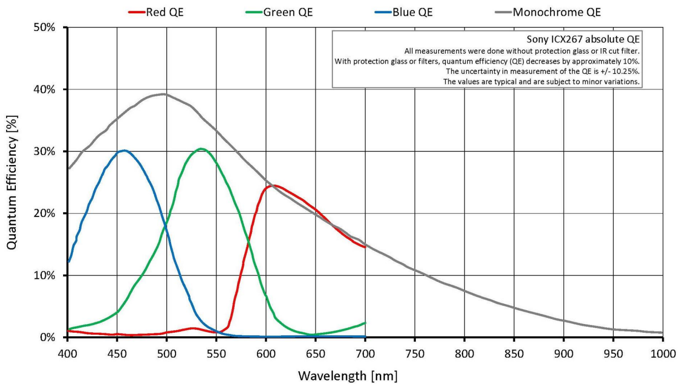
Quantum Efficiency
