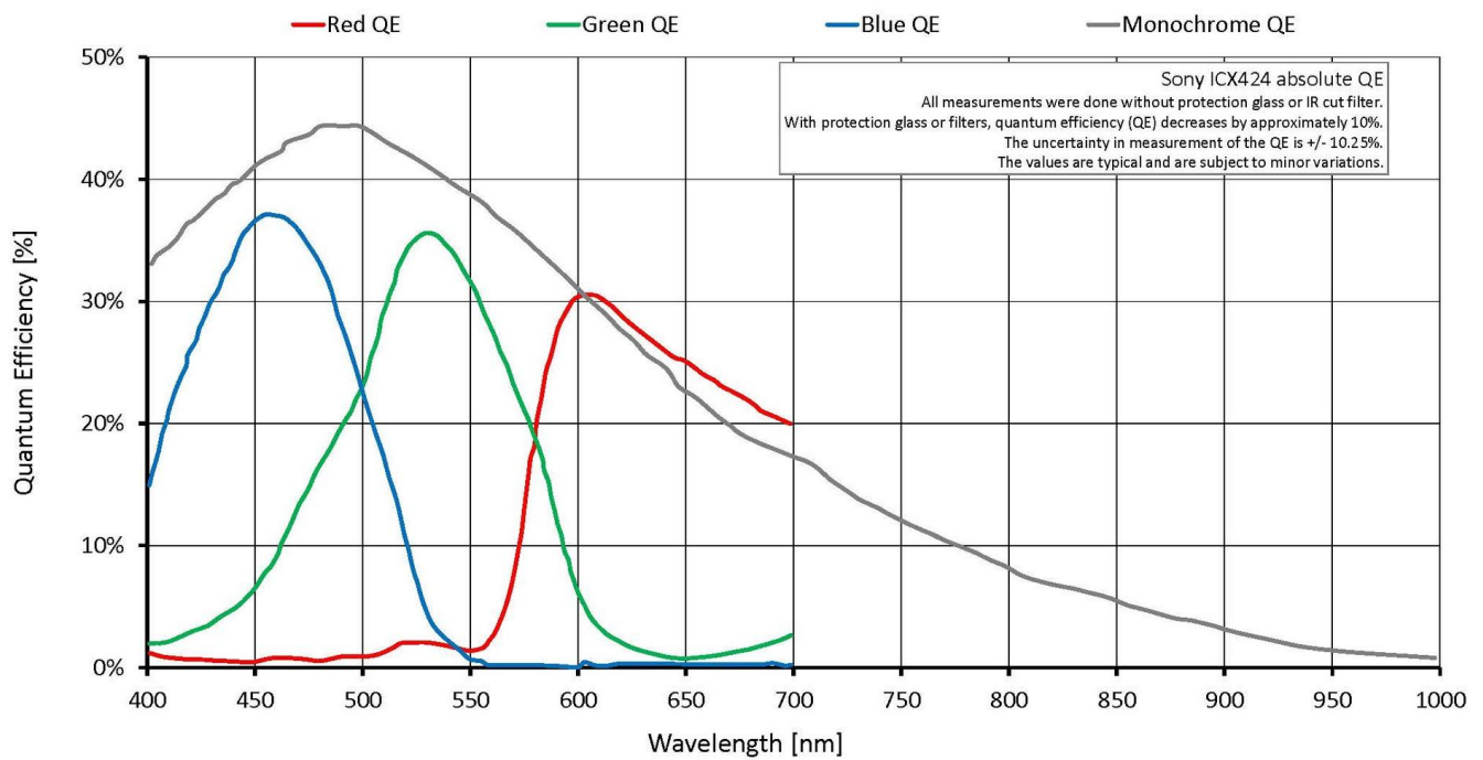
Quantum Efficiency
