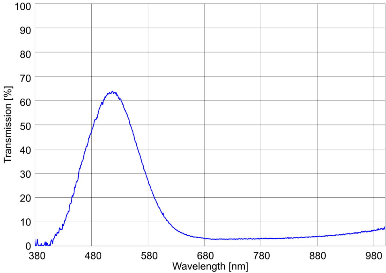
Transmission Colour Filter Green G06
