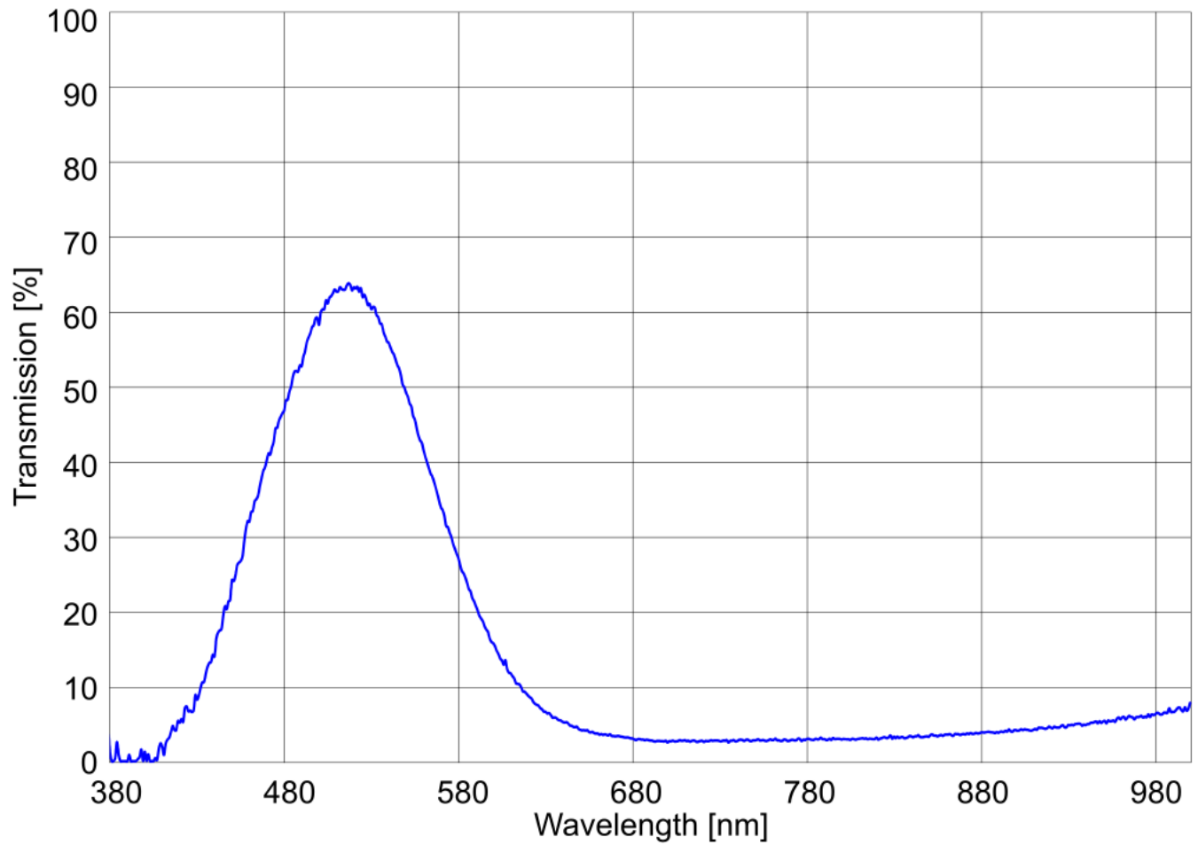
Transmission curve
