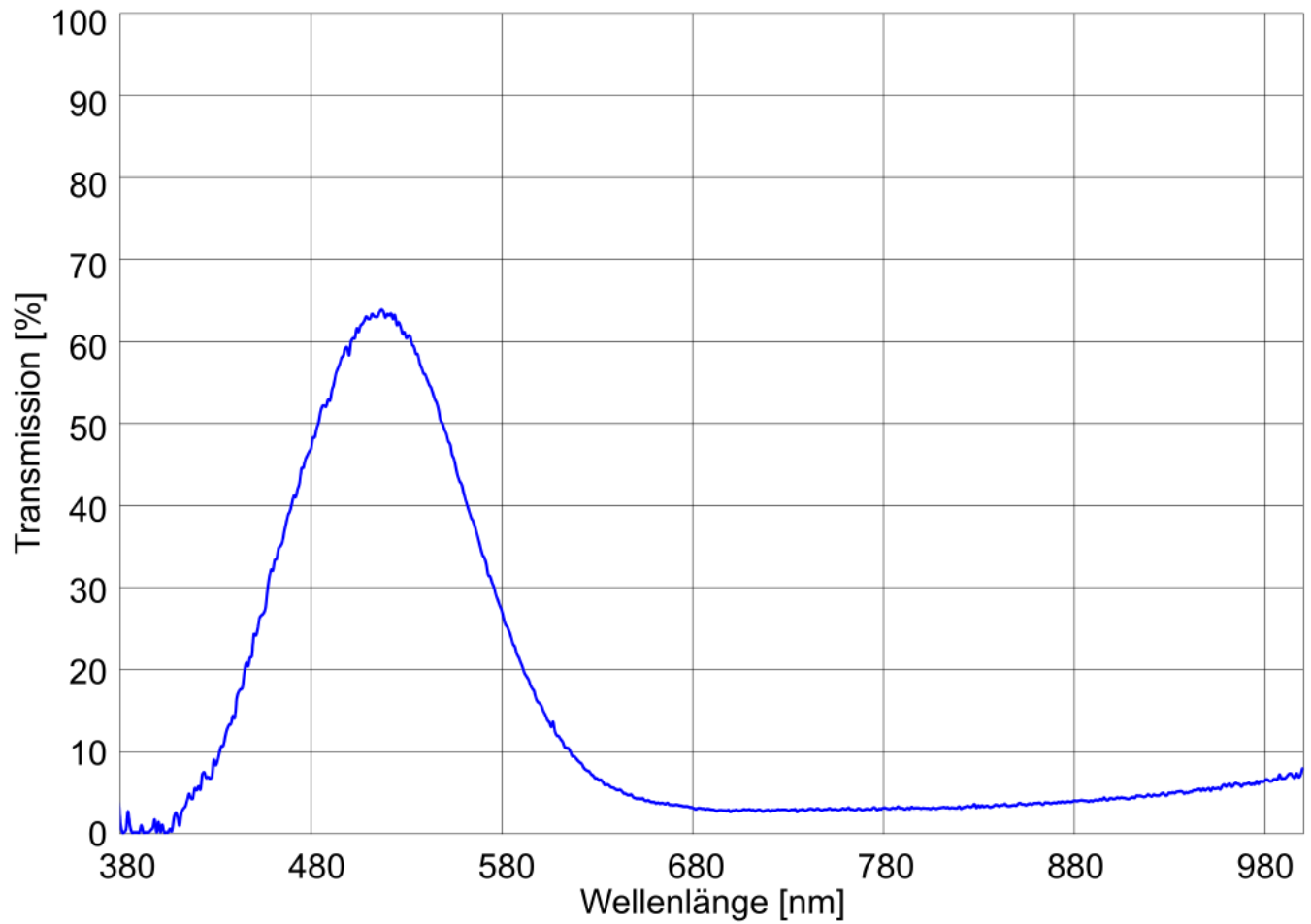
Transmissionskurve
