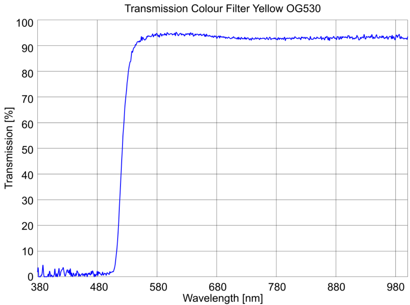
Transmission curve
