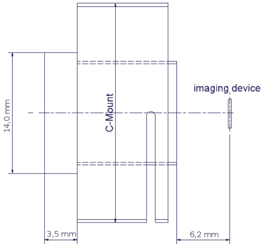
Dimensional drawing in mm
