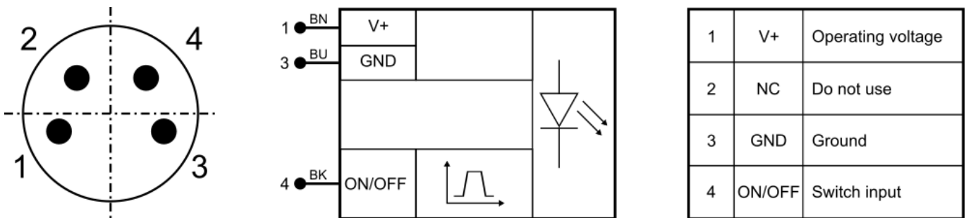
Pin assignment of the M8 connector
