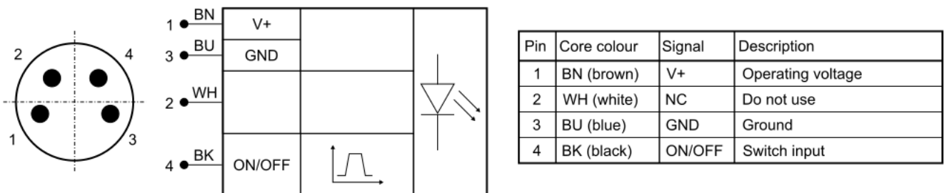
Pin assignment: M8 connector
