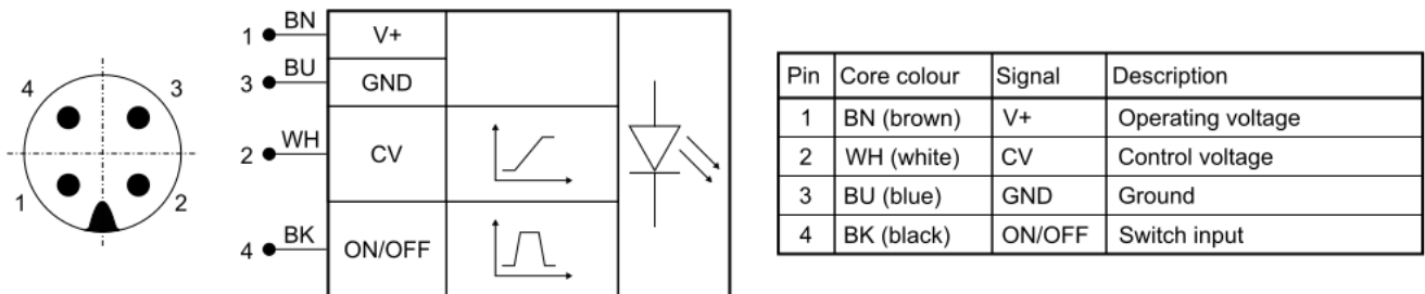
Pin assignments, M5 connector
