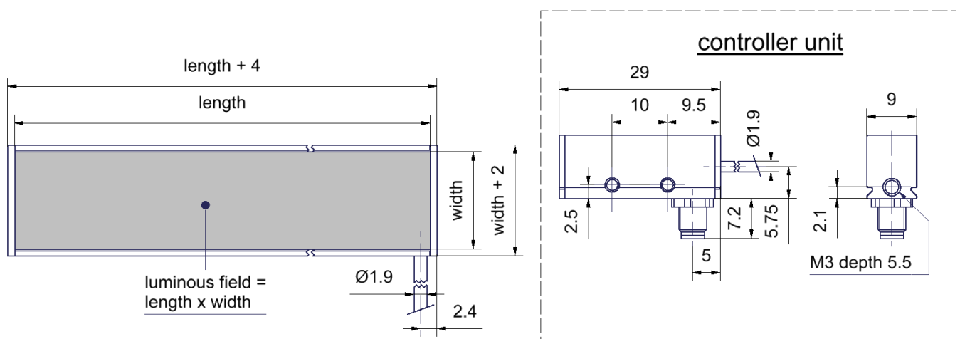
light unit
