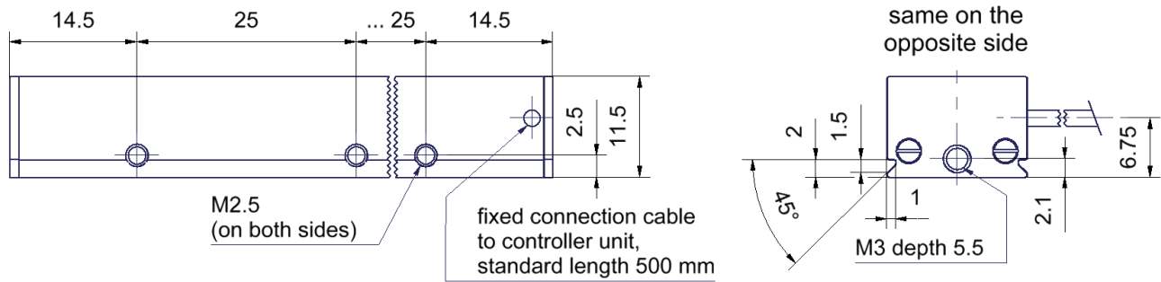
light unit
