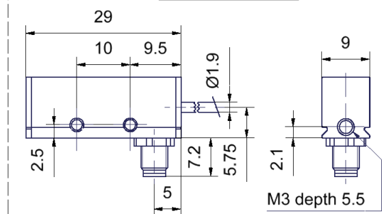
controller unit
