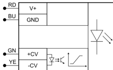
Pin assignment: cable open, 4-core
