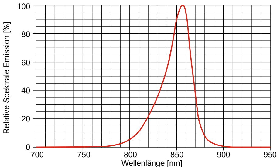
Abb. 4: Spektrale Emission
